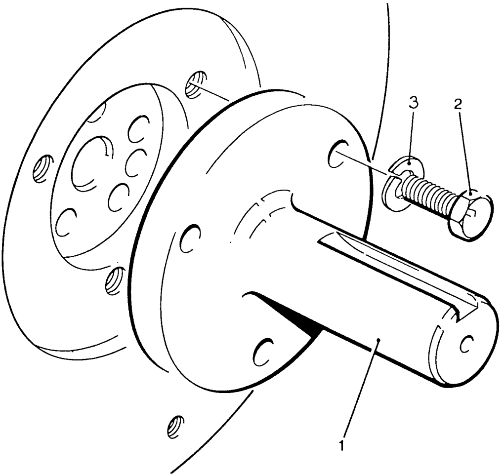
ALPHA RANGE FLYWHEEL END P.T.O. - LPA, LPW/S
